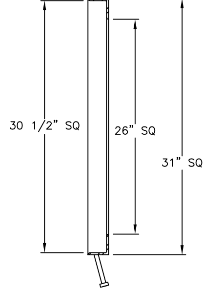
SECTION VIEW
