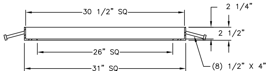
SECTION VIEW
